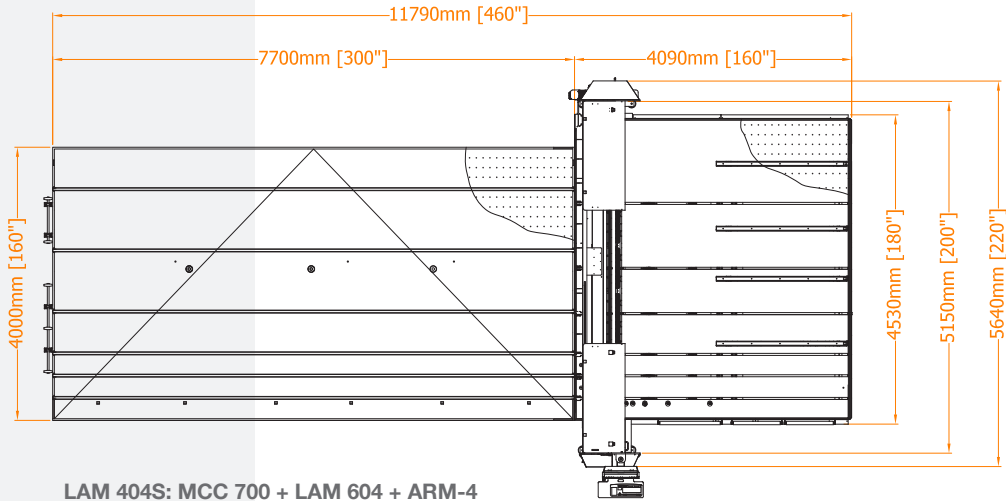
LAM 404S: MCC 700 + LAM 604 + ARM-4
