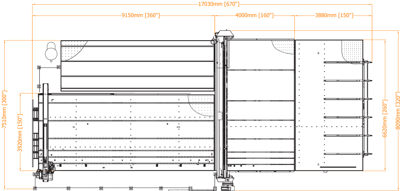
LAM 406TR: RUBI 306TC + AFLC-600 + LAM 406 + MC-300B5-4
