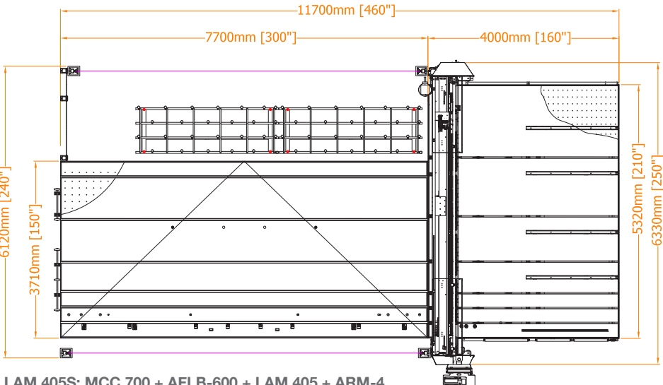
LAM 405S: MCC 700 + AFLB-600 + LAM 405 + ARM-4
