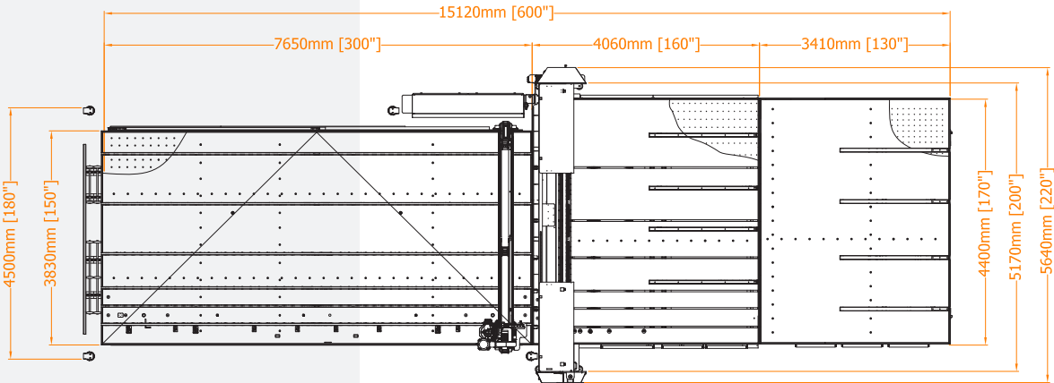
LAM 404TR: RUBI 306TC + LAM 404 + MC-300B4-4
