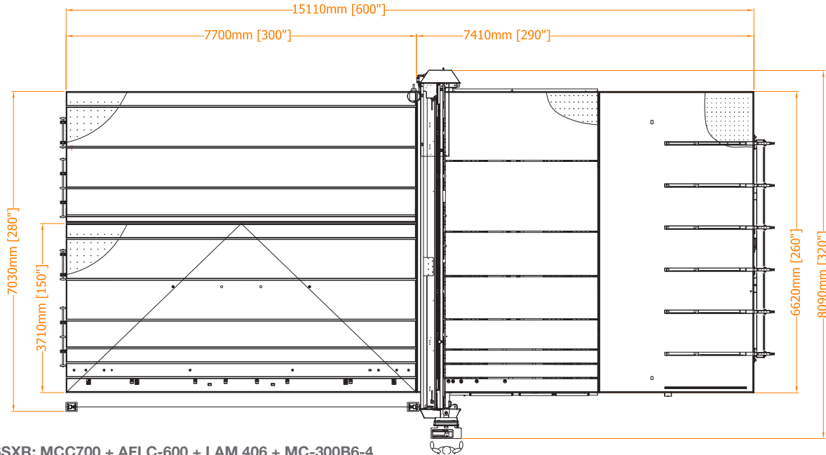
LAM 406SXR: MCC700 + AFLC-600 + LAM 406 + MC-300B6-4
