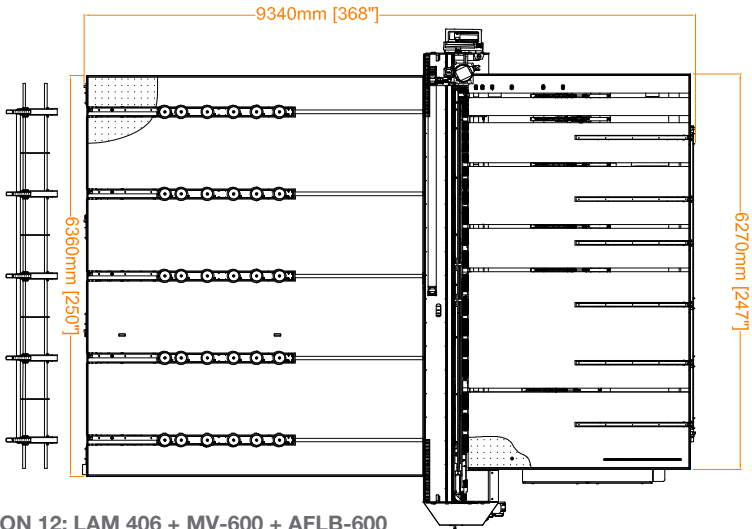
DISTRIBUTION 12: LAM 406 + MV-600 + AFLB-600
