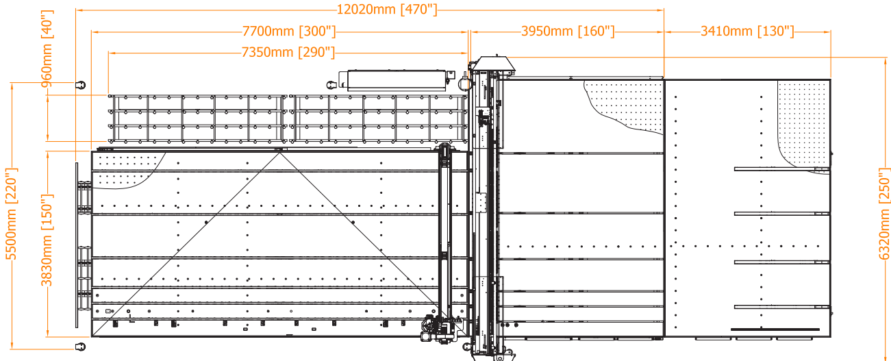
LAM 405TR: RUBI 306TC + LAM 405 + MC-300B5-4
