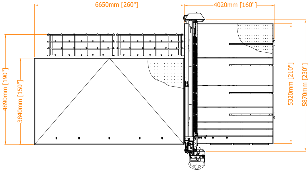
DISTRIBUTION 7: LAM 405 + MC-600 + AFLB-600
