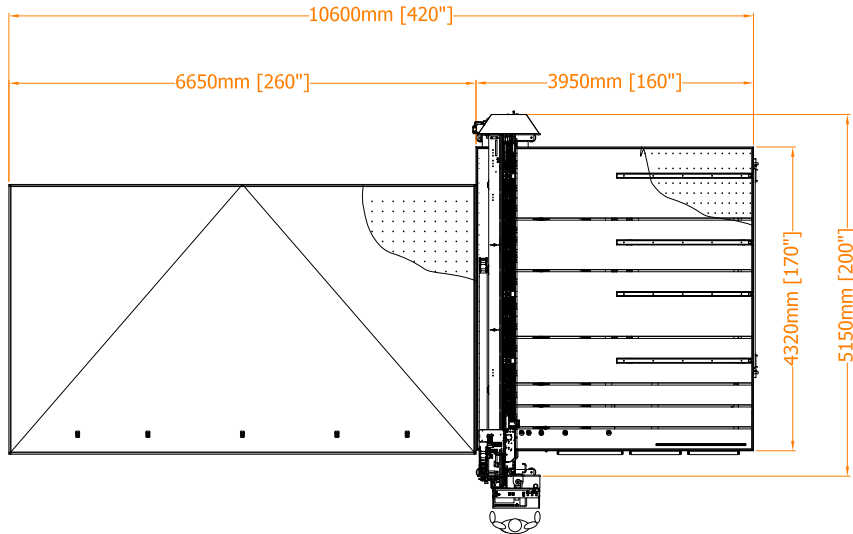
DISTRIBUTION 4: LAM 404 + MC-600
