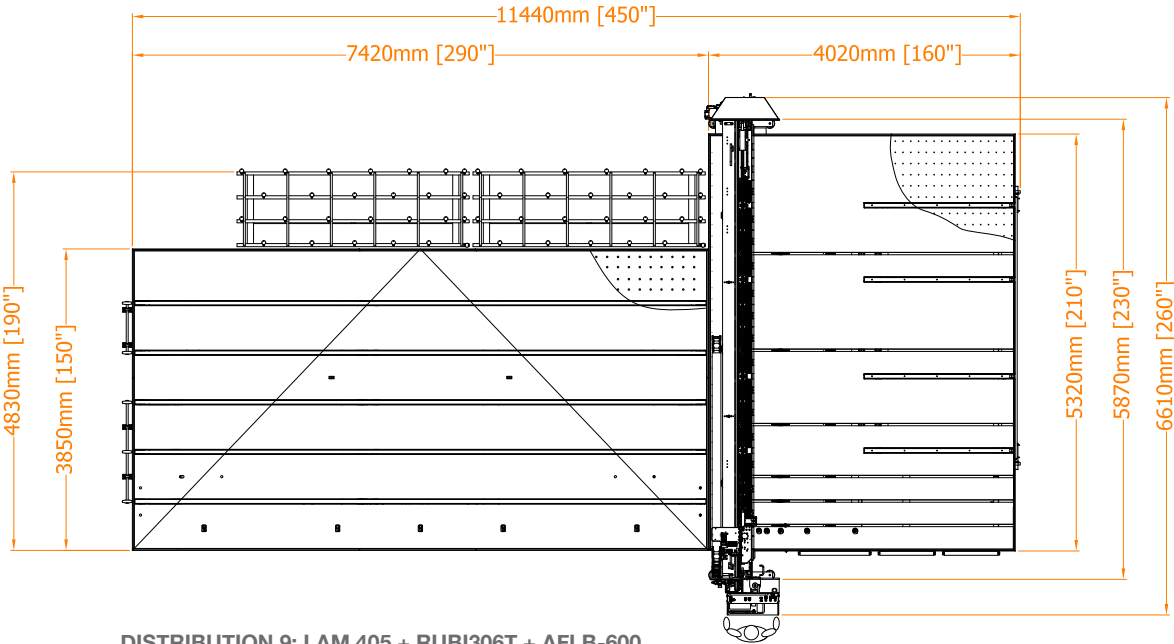
DISTRIBUTION 9: LAM 405 + RUBI306T + AFLB-600
