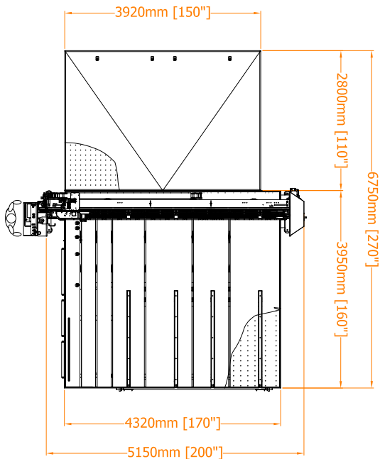
DISTRIBUTION 3: LAM 404 + MC-600
