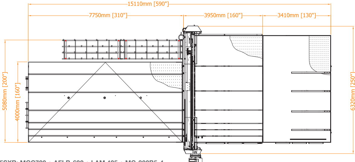
LAM 405SXR: MCC700 + AFLB-600 + LAM 405 + MC-300B5-4
