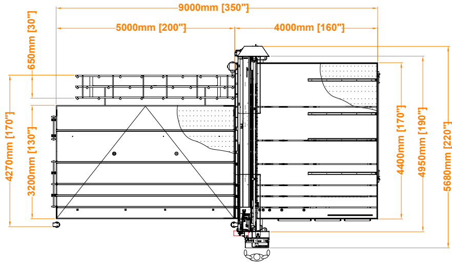
DISTRIBUTION 5: LAM 404 + MCC-400
