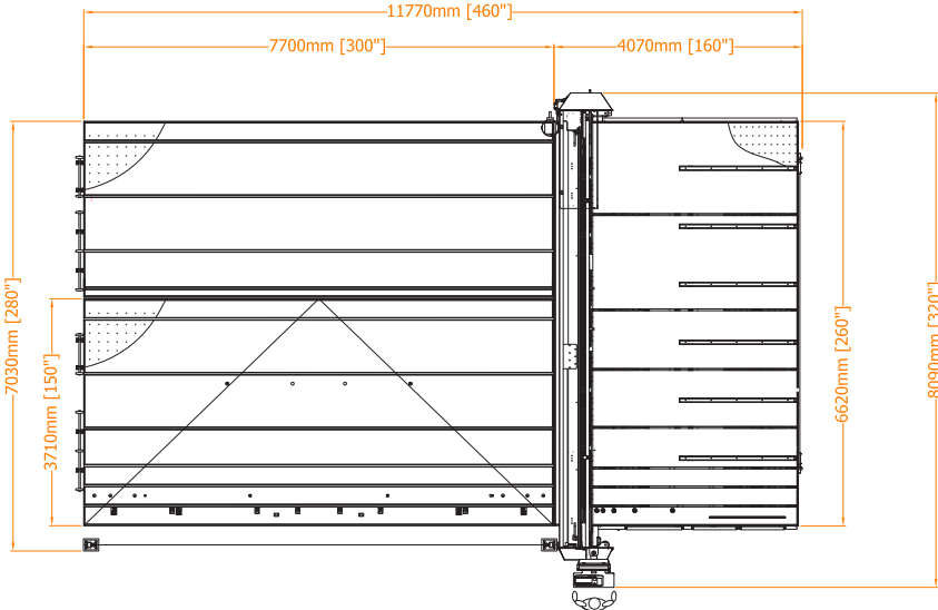
LAM 406S: MCC 700 + AFLC-600 + LAM 406 + ARM-6
