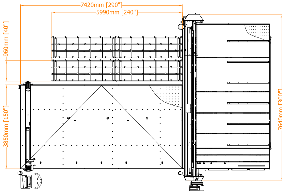
DISTRIBUTION 13: LAM 406 + RUBI306T + AFLB-600
