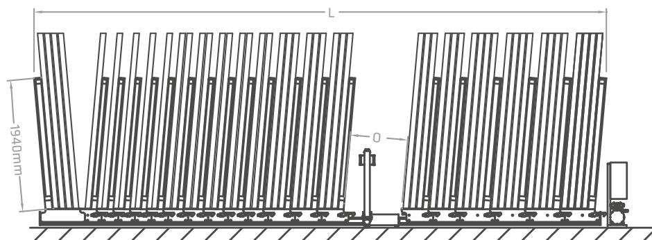
TILTING SECURITY SHAPE
